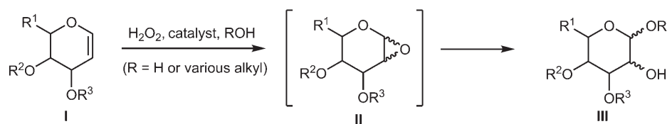
Scheme 1. Generalized reaction scheme for tandem epoxidation-alcoholysis or epoxidation-hydrolysis of variously protected glycals.
