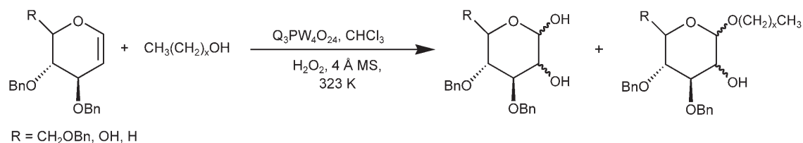
Scheme 2. General scheme for incorporation of long-chain alcohols with Venturello's compound.
